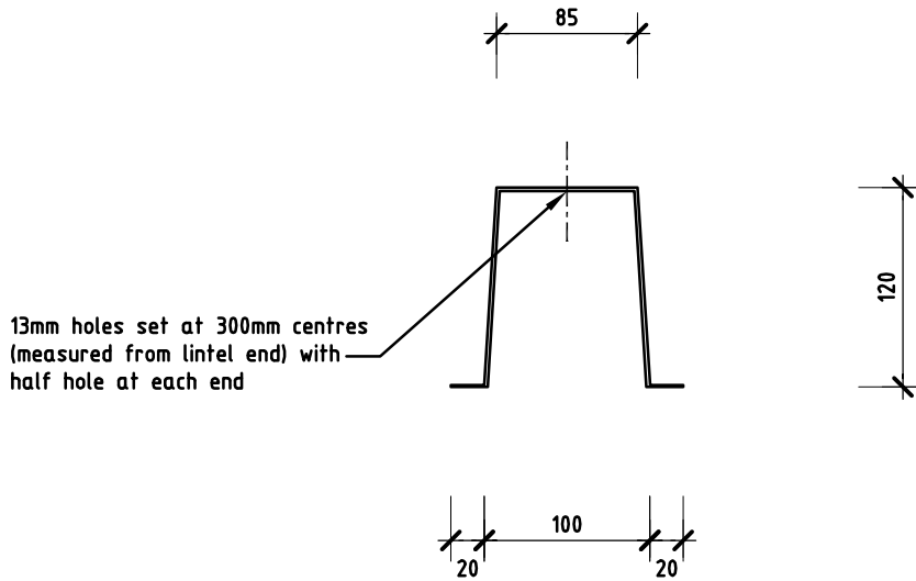
Figure 01 - Dimensions
